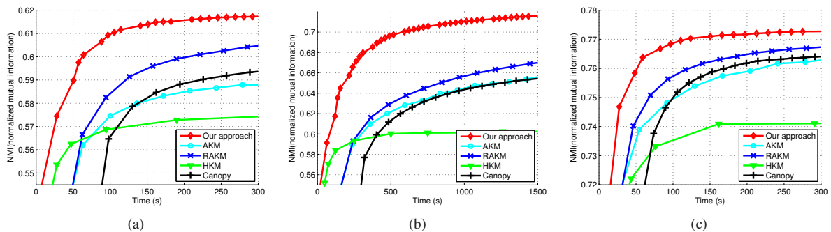
Figure 7. Clustering performance in terms of normalized mutual information (NMI) vs. time, on the dataset of (a) 200K tiny images, (b) 500K tiny images, and (c) 200K shopping images.
